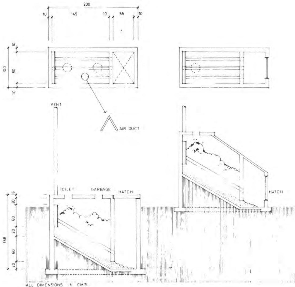
The Minimus composting toilet (from 2224).
