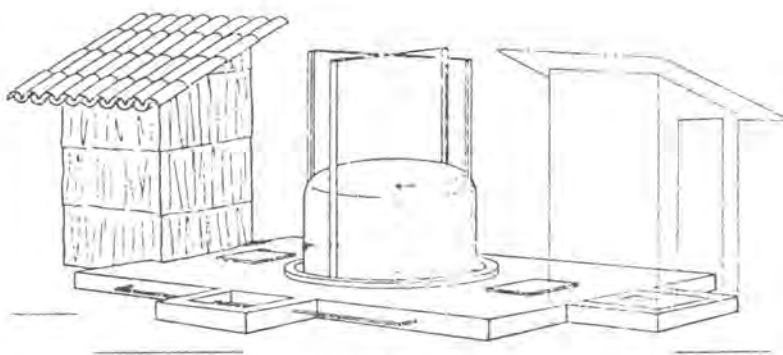
The excreta-fed biogas plant (from 4520).
