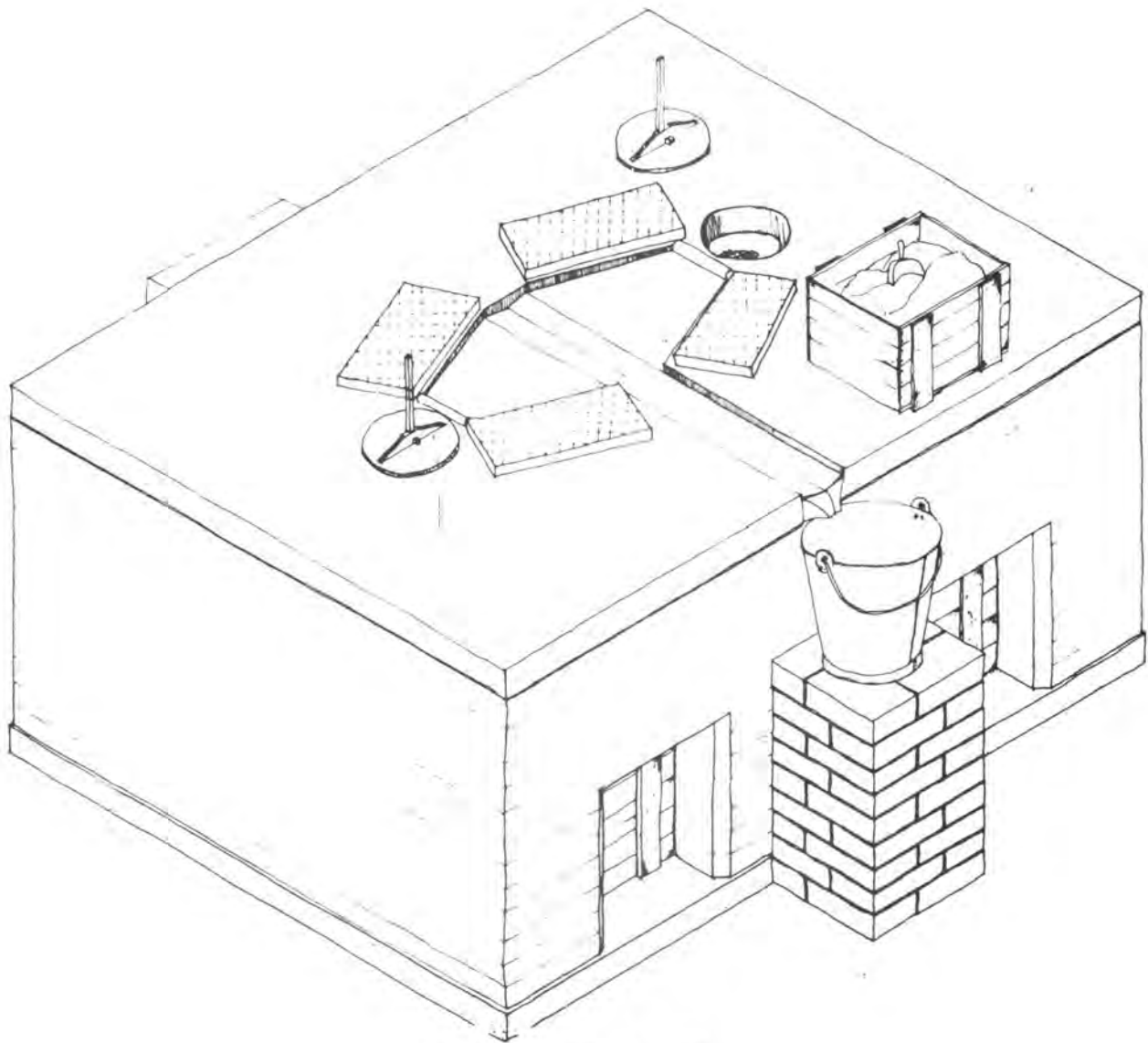
The Vietnamese double vault.
