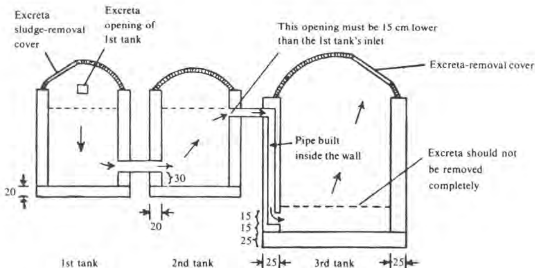
The Chinese three-tank toilet (from 2303).
