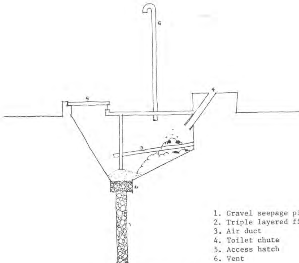
The biopit composting toilet (from 2219).
