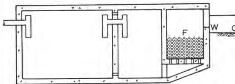
The septic tank with upflow filter (from 2356): F, filter; W, effluent weir; C, effluent channel.
