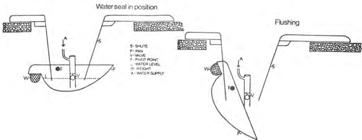
The Watergate flushing pan (from 1008).
