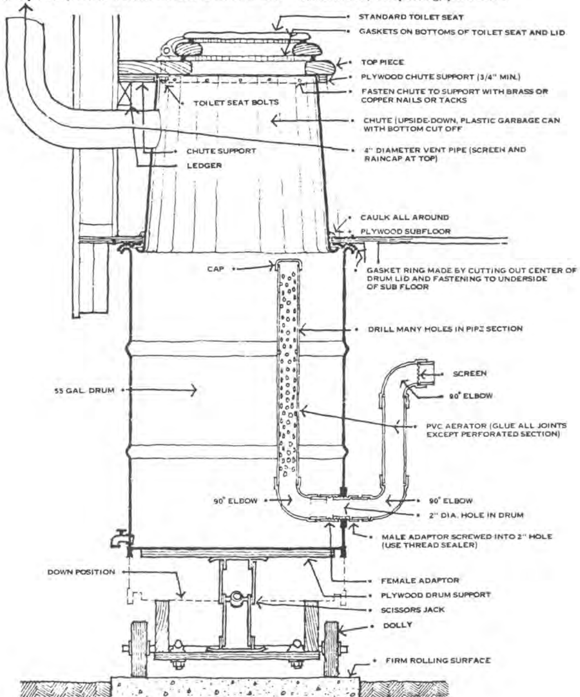
Matson drum privy (from 2135).
