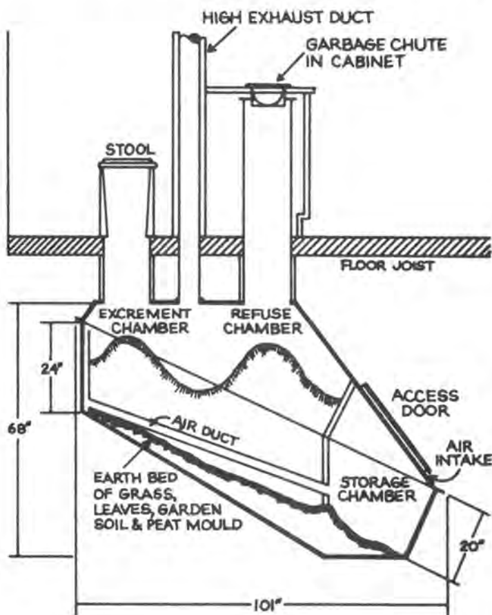
Cross section of the Clivus Multrum
