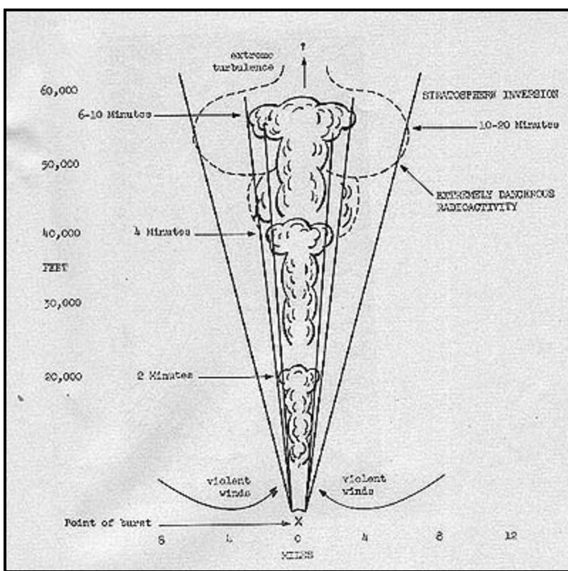
FIGURE 1 Probable position of rising cloud at intervals after explosion
