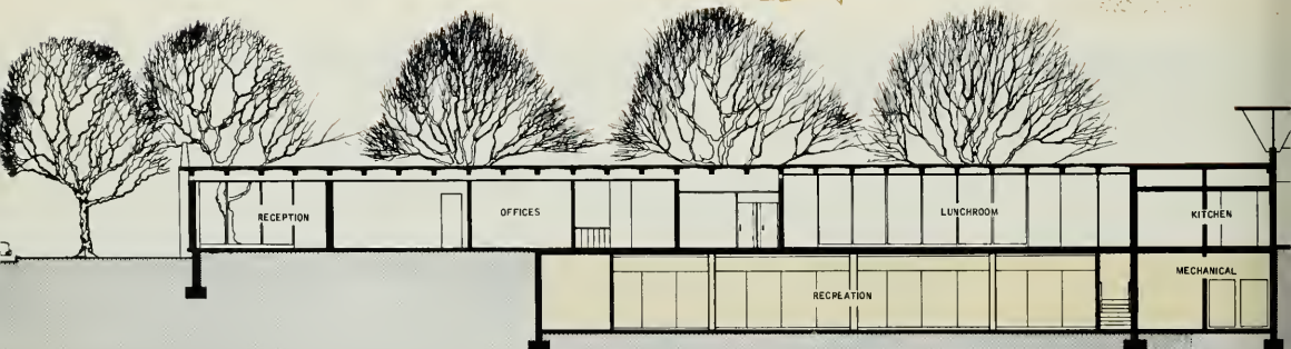
LONGITUDINAL SECTION SHOWING BASEMENT SHELTER
