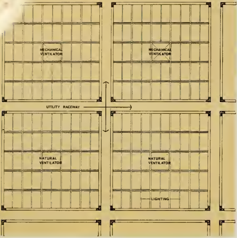
REFLECTED CEILING PLAN 0 2.4 4.8 9.6
