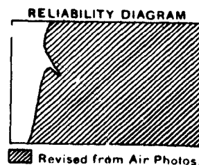
Figure 10. Reliability diagram.
