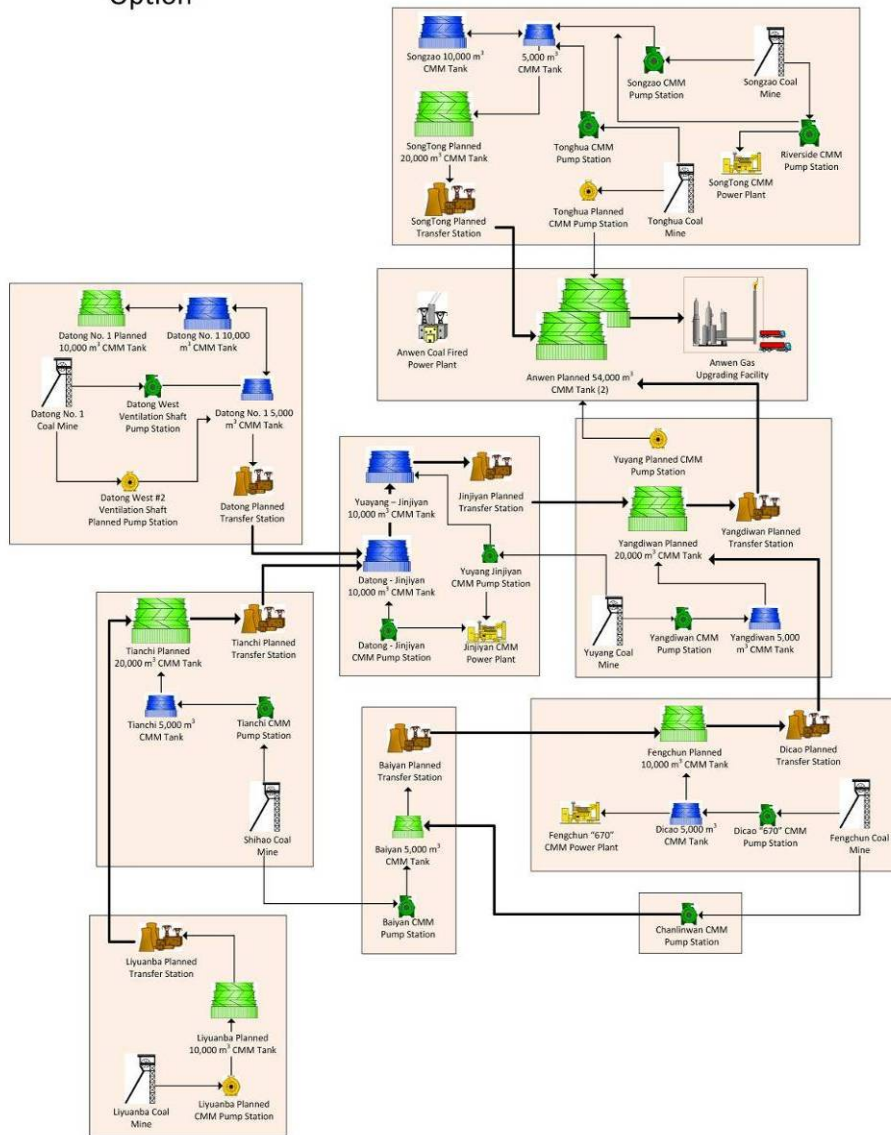
FIGURE 32: BLOCK FLOW DIAGRAM FOR CONCEPTUAL DESIGN OF LNG ONLY OPTION
