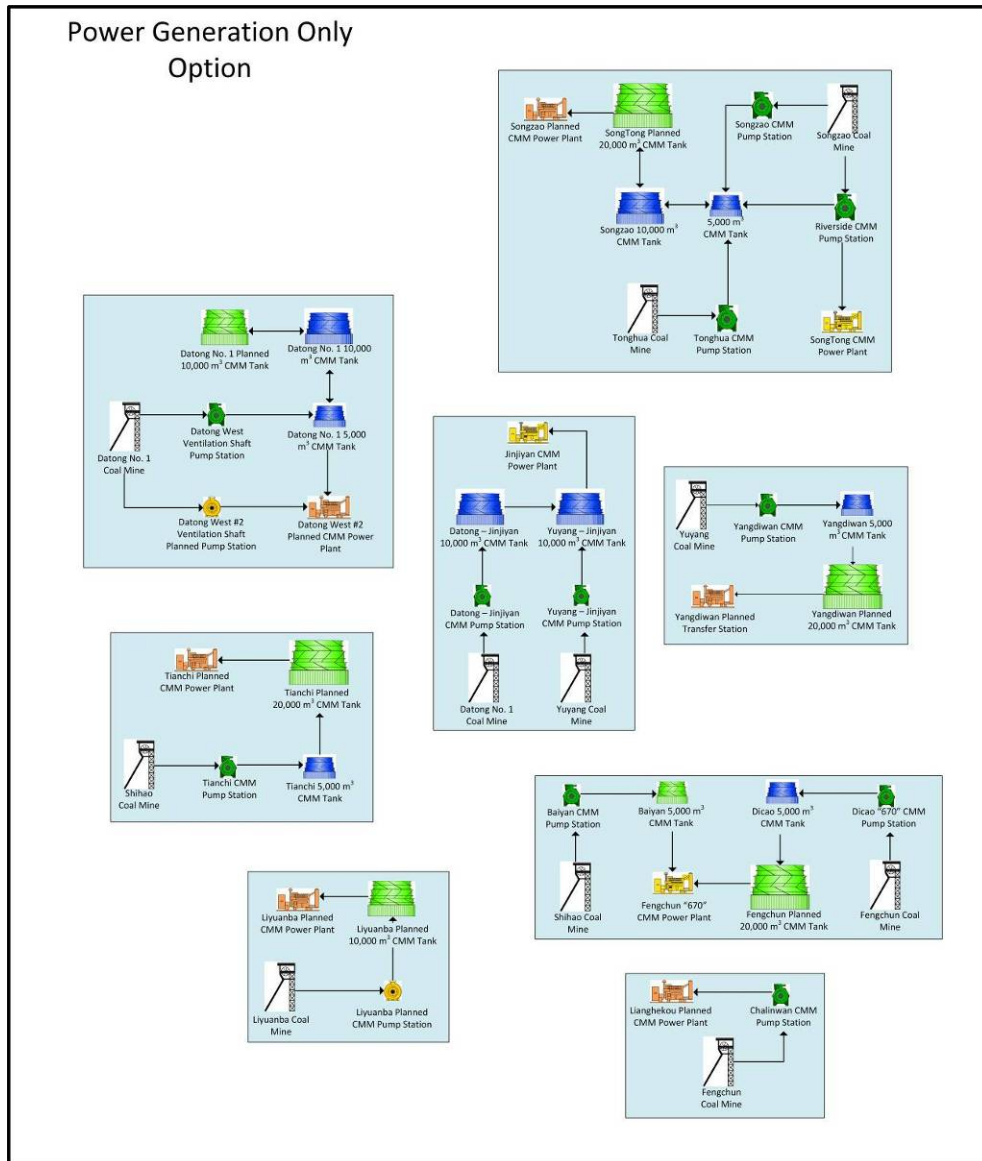
FIGURE 31: BLOCK FLOW DIAGRAM FOR CONCEPTUAL DESIGN OF POWER GENERATION ONLY OPTION
