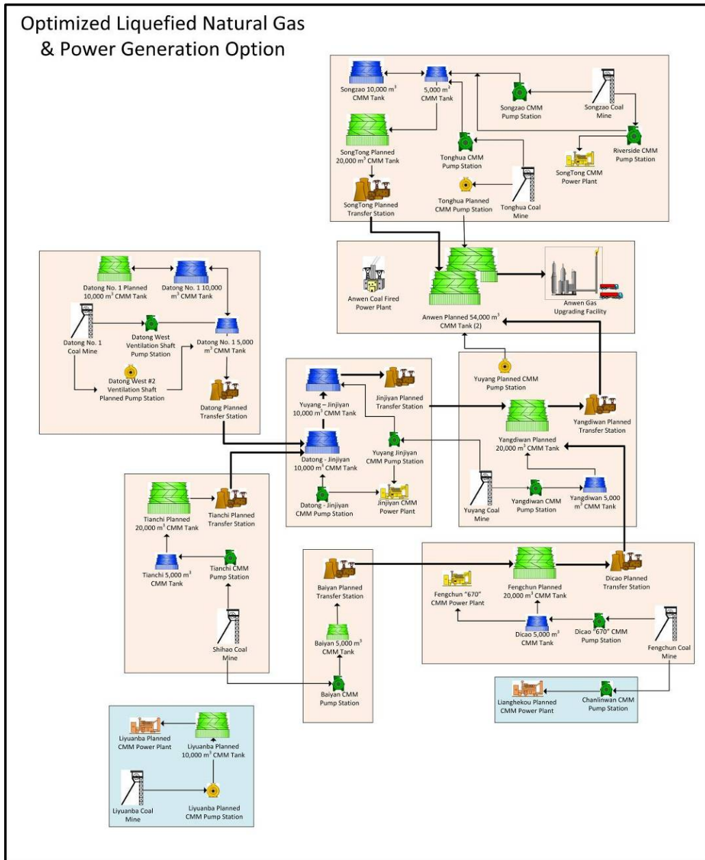
FIGURE 34: BLOCK FLOW DIAGRAM FOR CONCEPTUAL DESIGN OF OPTIMIZED OPTION
