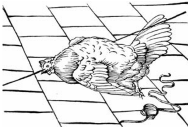
SCHWENTER'S HEN EXPERIMENT, REPRODUCED BY FATHER ATHANASIUS KIRCHER.
