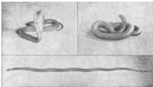
THE EGYPTIAN SNAKE NAJA HAJA MADE MOTIONLESS BY PRESSURE ON THE NECK. [133] (Reproduced from Verworn after photographs.)
