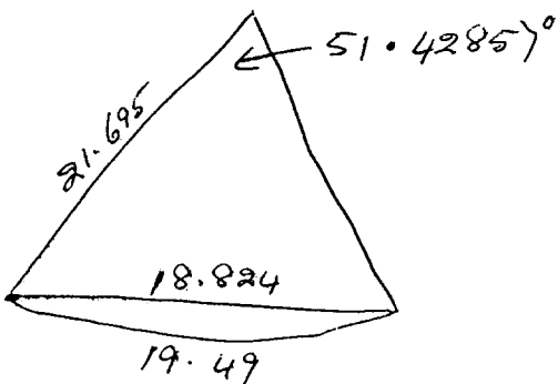
PLAN VIEW OF ONE SEGMENT.
